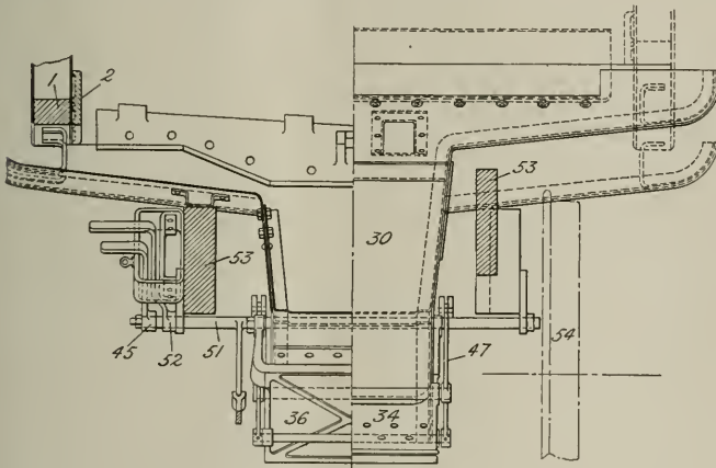
FURTHER DETAILS OF ASHPAN
